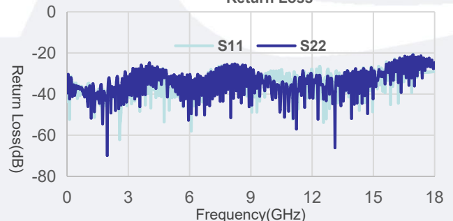
A81-NWMNWM-1m Return Loss
