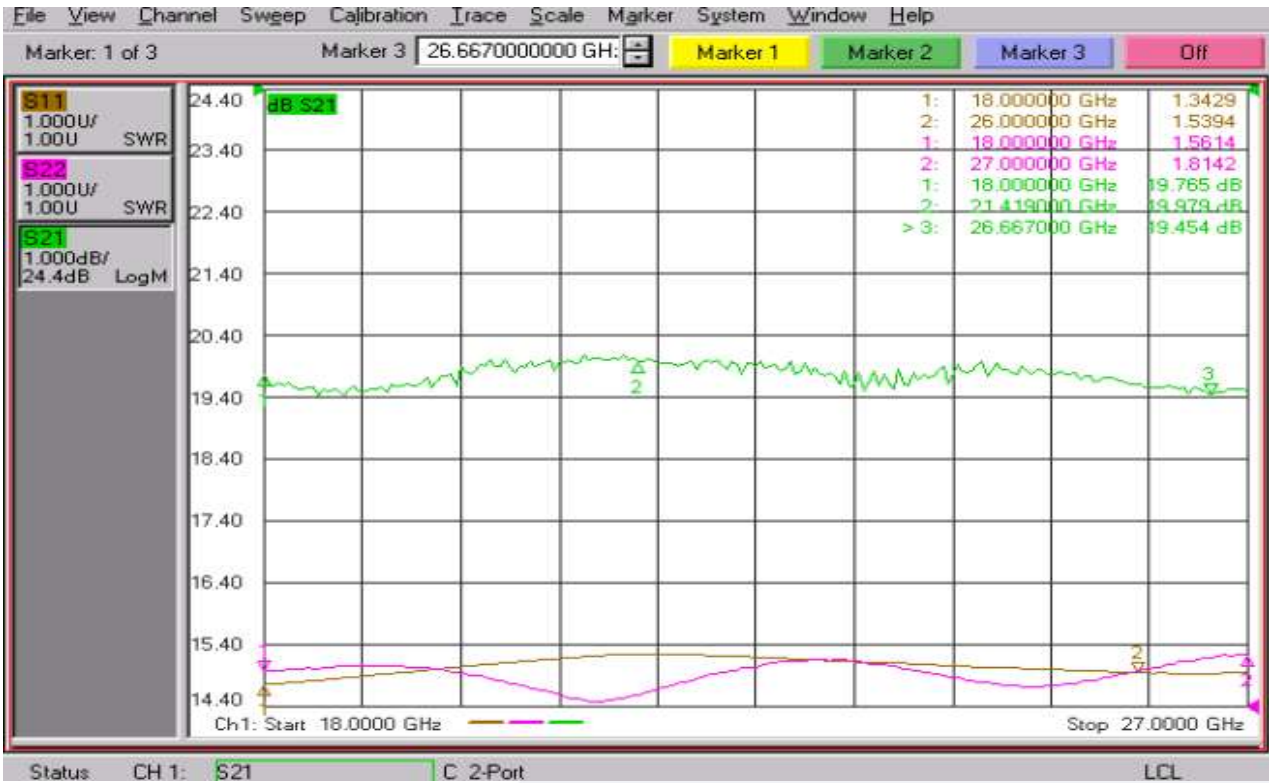
Gain&VSWR VS. Frequency
