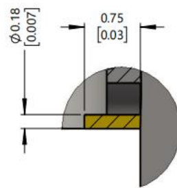
DETAIL A(20:1)
