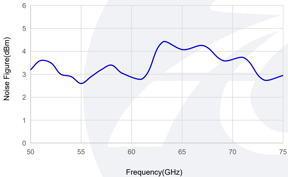
Noise Figure vs Frequency
