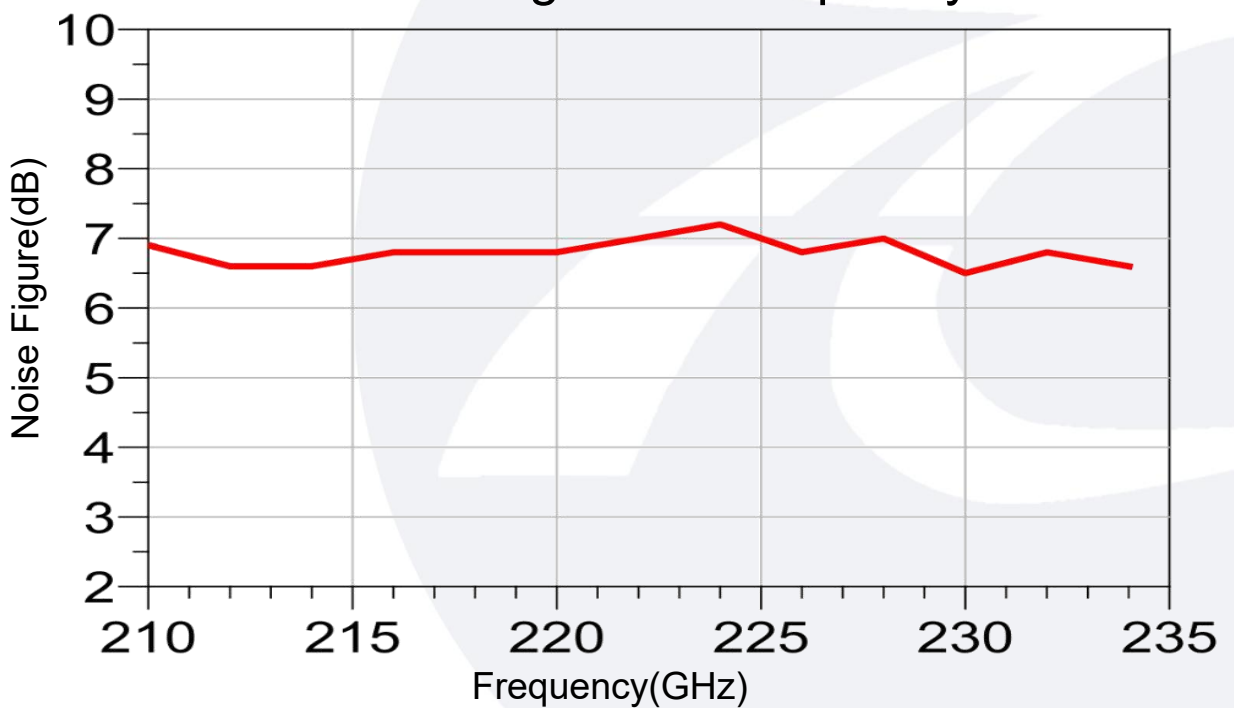
Noise Figure vs Frequency
