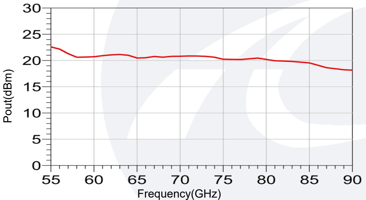
Psst vs Frequency@Pin=2dBm
