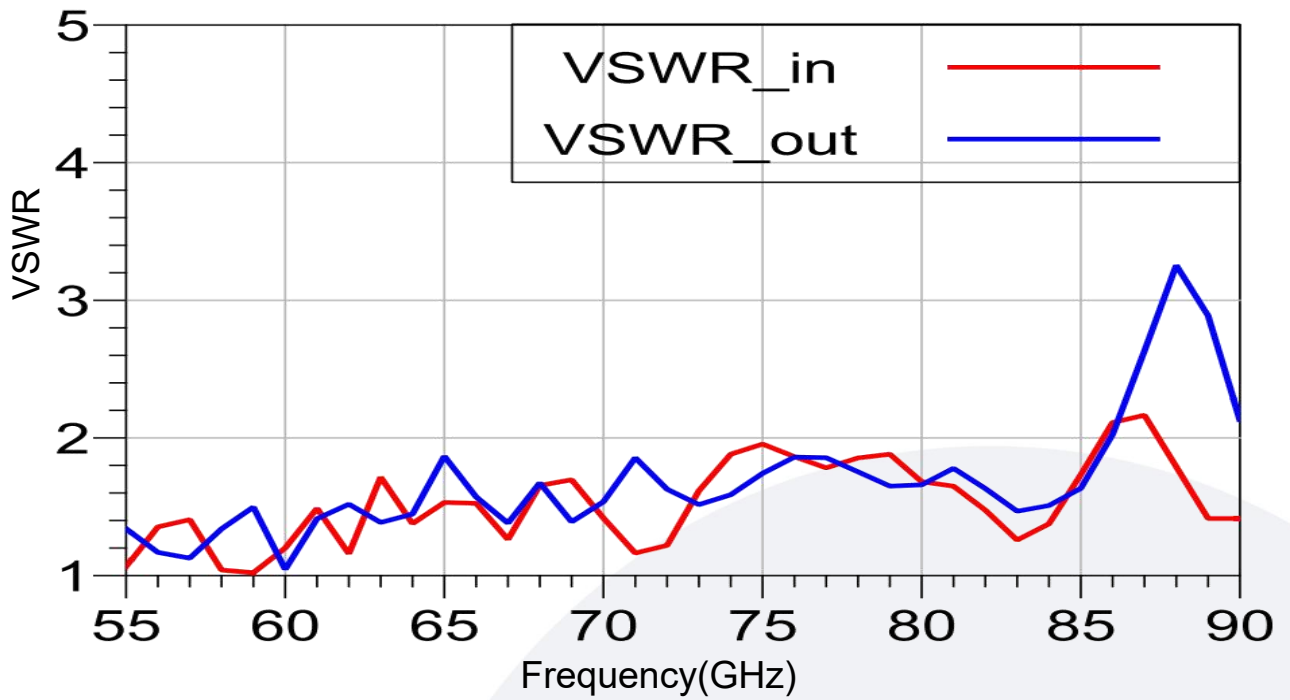
VSWR vs Frequency
