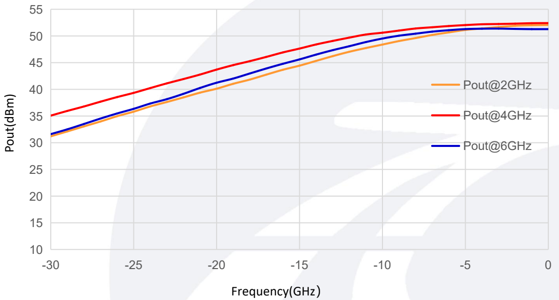
Pout@Pin vs Frequency
